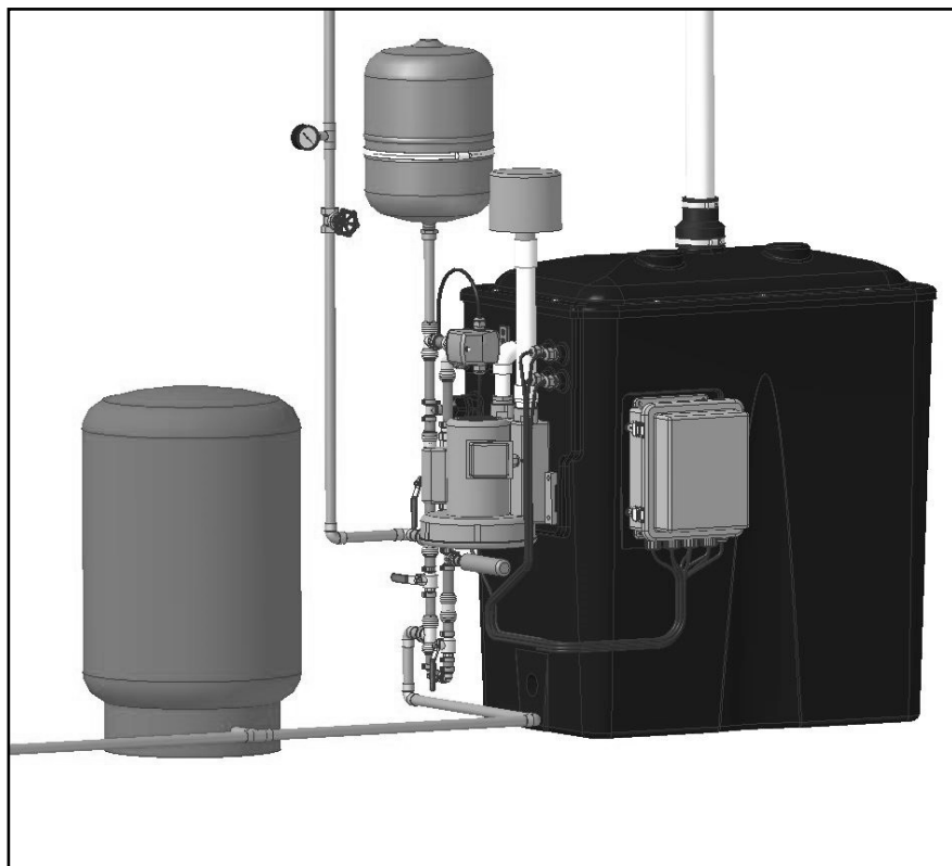
Figure 15 Installed AIRaider™ 433-S50
